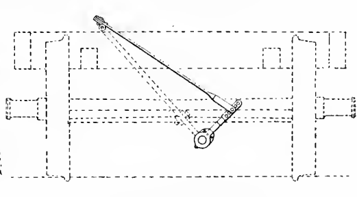
THE HINCKLEY BRAKE SLACK ADJUSTER EQUIPMENT D.
